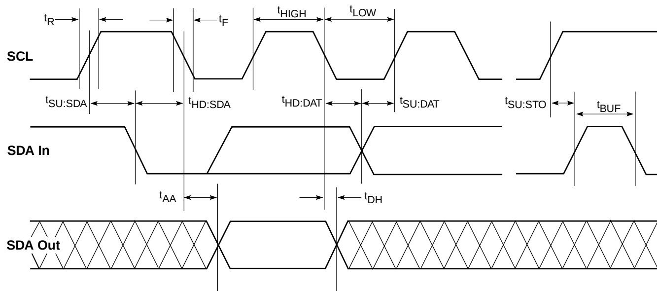
Figure 11. Bus Timing
