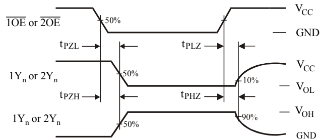
Figure 2. Switching Waveforms
