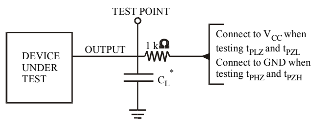
Figure 4. Test Circuit
