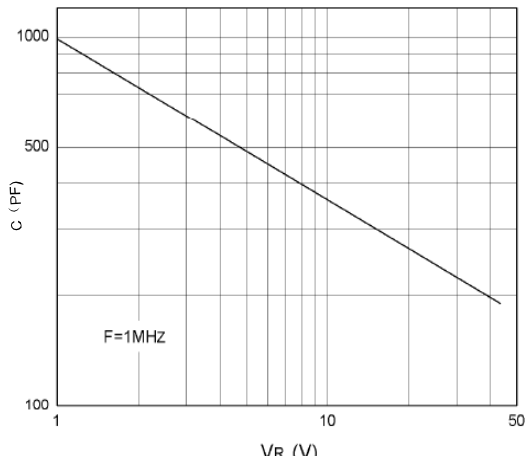
Fig.3 Junction capacitance versus reverse voltage applied (typical values, per diode).
