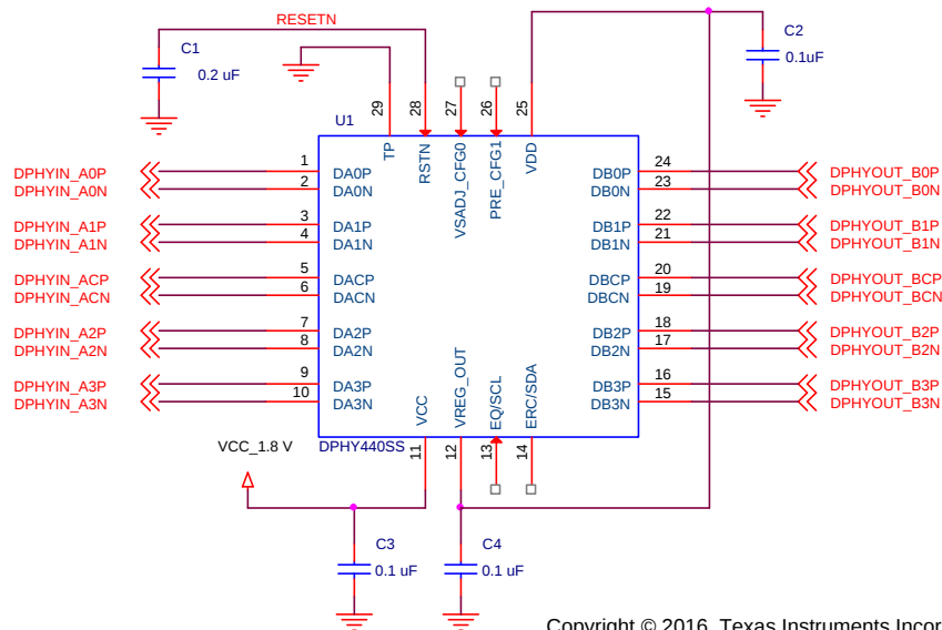
Figure 24. Supply Implementation
