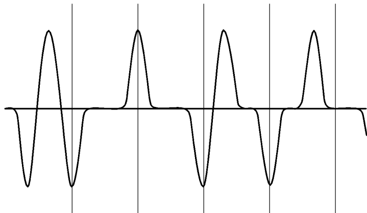
FIGURE 3. Typical AMI Waveform at L_0
