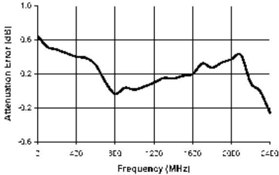
Attenuation Error, 16 dB Bit
