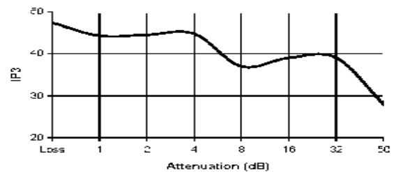
Maximum IP3 over Temperature Range and Attenuation @ 950 MHz
