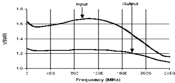
VSWR, 8 dB Bit
