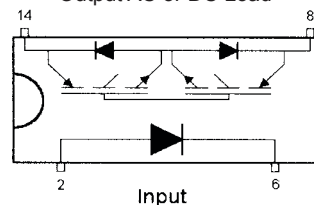
Connection Diagram Output AC or DC Load
