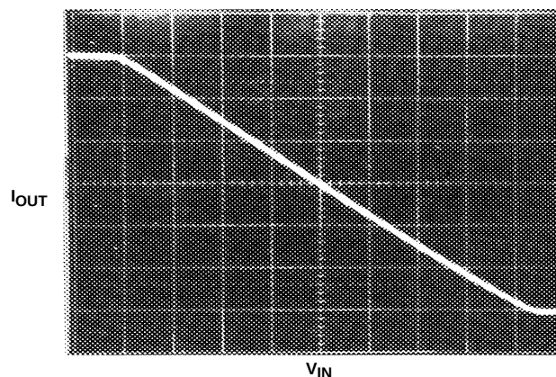
FIGURE 3A. EFFECTS OF DIODE LINEARIZATION, WITH DIODE PROGRAMMING TERMINAL ACTIVE
