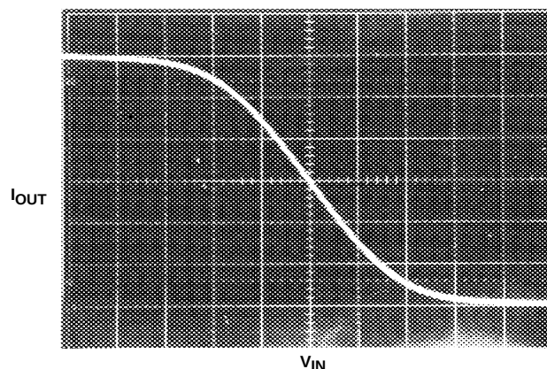
FIGURE 3B. WITH DIODE PROGRAMMING TERMINAL CUTOFF
