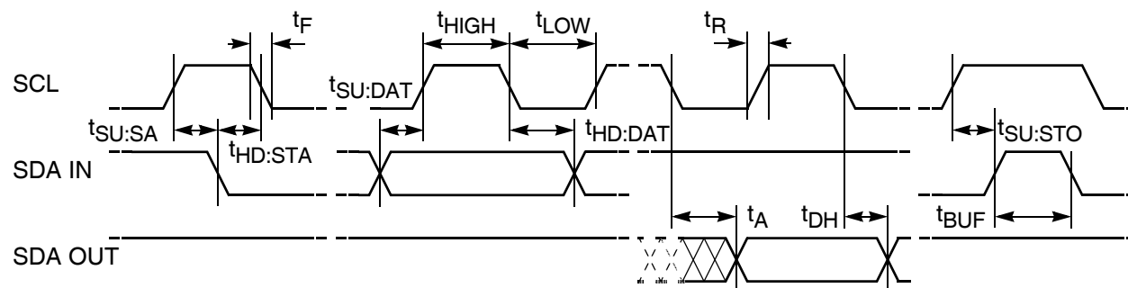
Figure 20. Bus Timing
