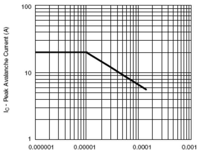
Single Pulse Avalanche Capability
