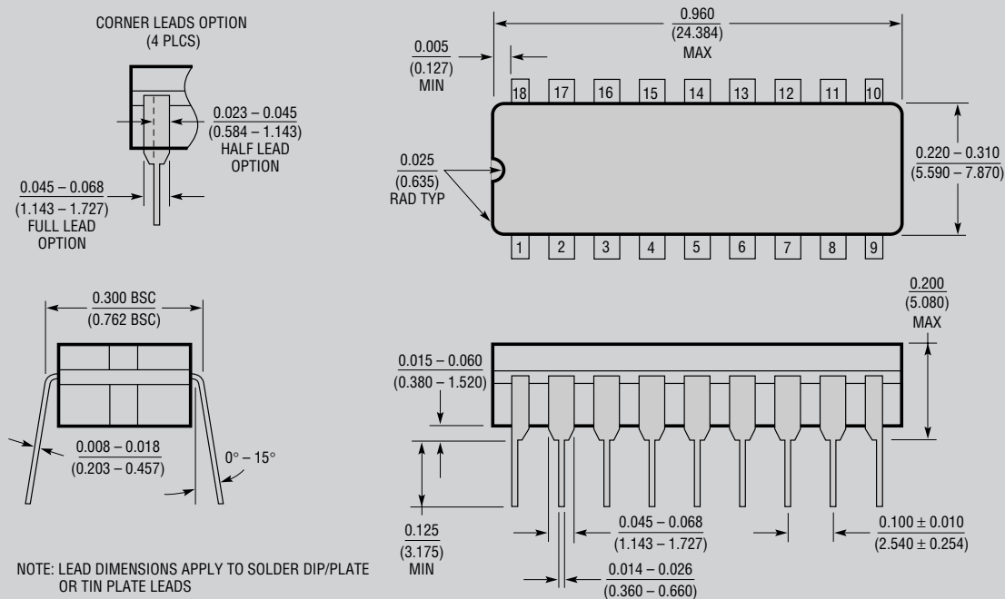
J Package 18-Lead CERDIP (Narrow 0.300, Hermetic) (LTC DWG # 05-08-1110)
