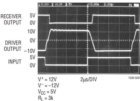
Output Waveforms
