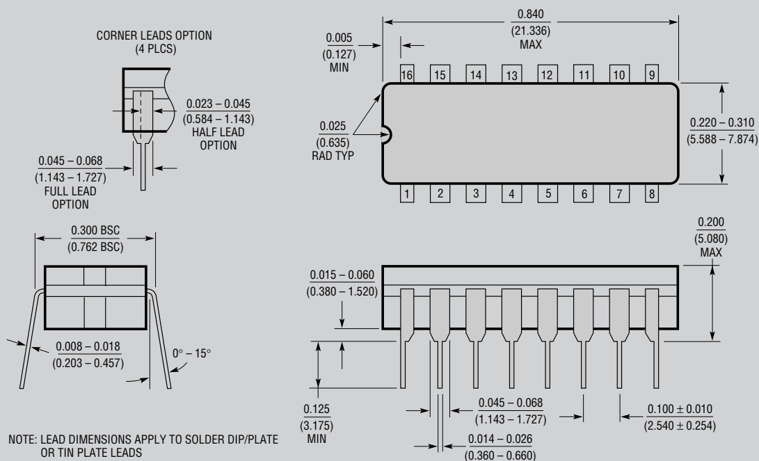
J Package 16-Lead CERDIP (Narrow 0.300, Hermetic) (LTC DWG # 05-08-1110)
