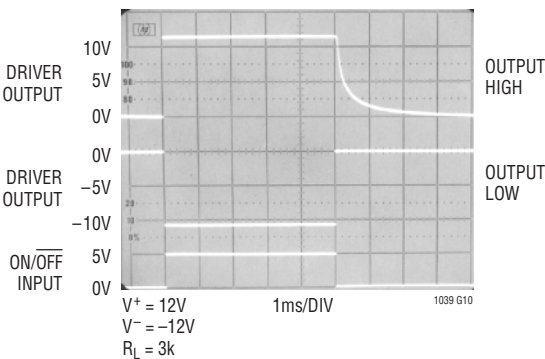
Shutdown to Driver Output
