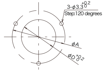
Mounting Dimensions
