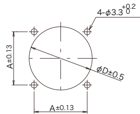
Mounting Dimensions
