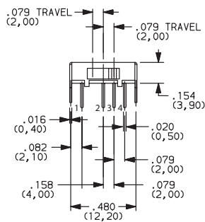
OS103011MA7QP1 SP3T
