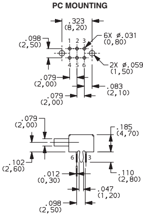
OS202011MA0QN1 DPDT
