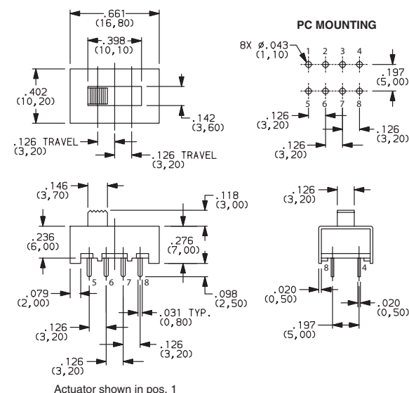
OS203013MT8QN1 DP3T
