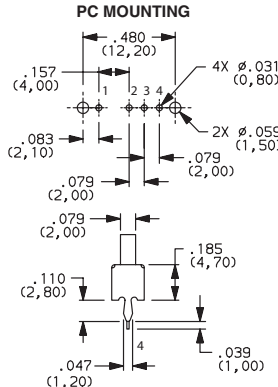
OS103011MS8QP1 SP3T
