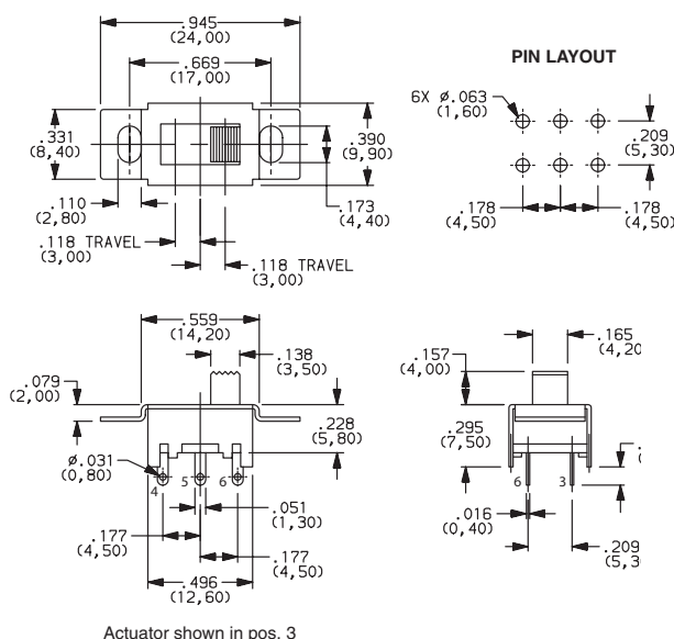
OS203013MT7QN1 DP3T
