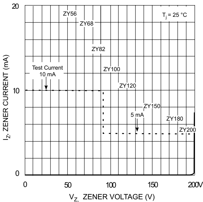
Fig. 3 Zener Breakdown Characteristics
