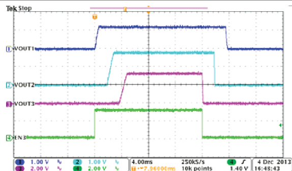
图 8-27. Automatic Power Sequencing, MODE = EN1 = EN2 = HIGH
