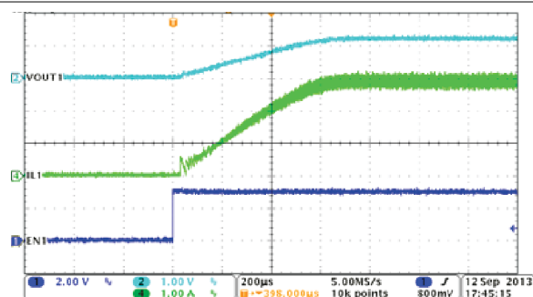
图 8-4. Buck1, Soft-Start With Full Load
