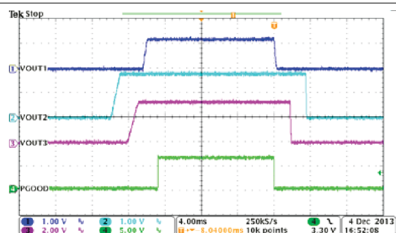
图 8-30. Automatic Power Sequencing, MODE = EN1 = HIGH, EN2 = LOW
