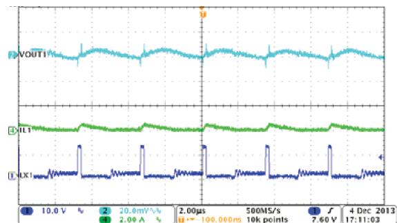
图 8-9. Buck1, Steady State Operation With Light Load
