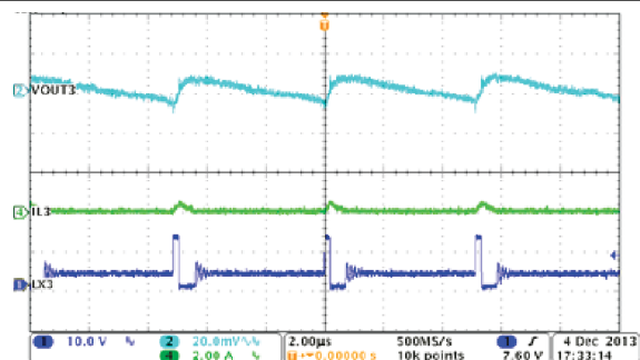
图 8-13. Buck3, Steady State Operation With Light Load
