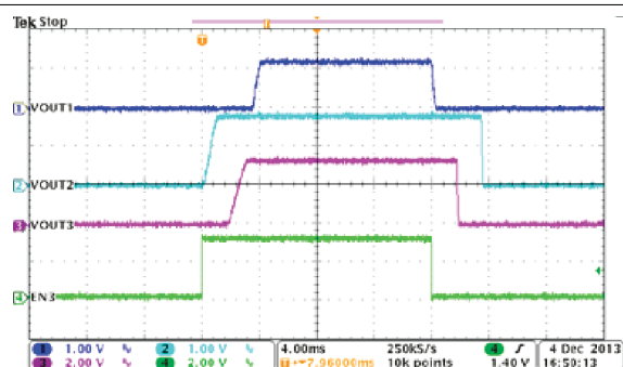
图 8-29. Automatic Power Sequencing, MODE = EN1 = HIGH, EN2 = LOW
