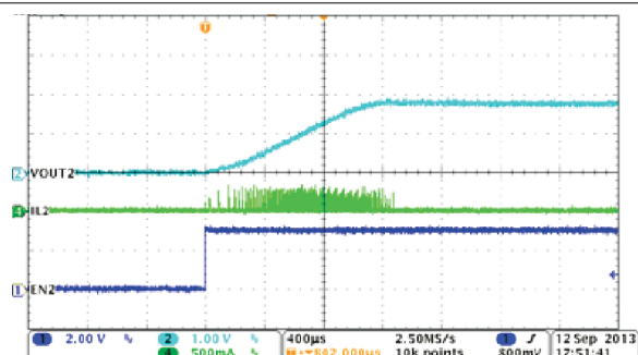
图 8-5. Buck2, Soft-Start With No Load
