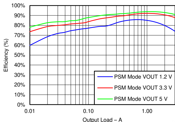
图 6-1. Buck1 Efficiency
