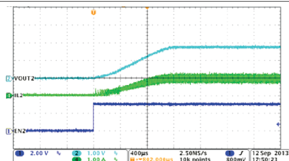
图 8-6. Buck2, Soft-Start With Full Load
