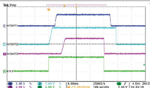
图 8-31. Automatic Power Sequencing, MODE = EN2 = HIGH, EN1 = LOW
