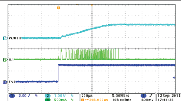
图 8-3. Buck1, Soft-Start With No Load
