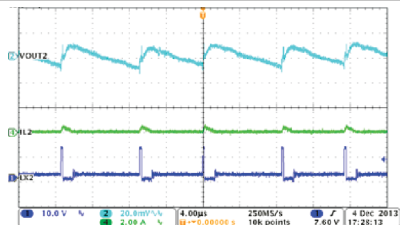
图 8-11. Buck2, Steady State Operation With Light Load
