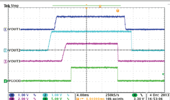
图 8-32. Automatic Power Sequencing, MODE = EN2 = HIGH, EN1 = LOW
