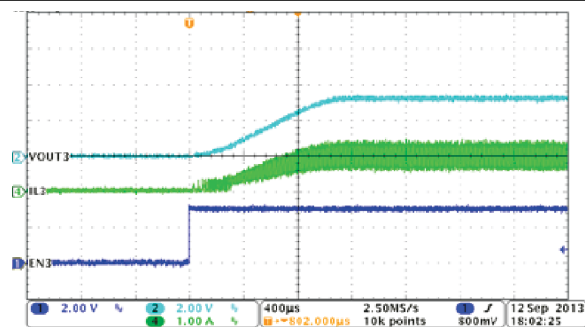
图 8-8. Buck3, Soft-Start With Full Load
