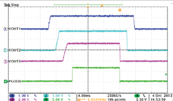
图 8-28. Automatic Power Sequencing, MODE = EN1 = EN2 = HIGH
