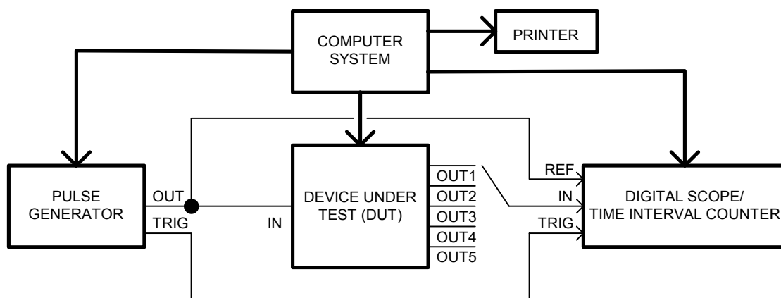
Figure 2: Test Setup
