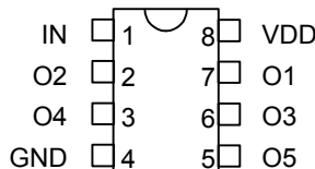
3D7205M DIP 3D7205H Gull-Wing
