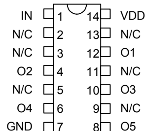
3D7205 DIP 3D7205G Gull-Wing 3D7205K Unused pins removed
