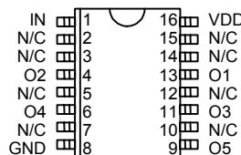
3D7205S SOL (300 Mil)
