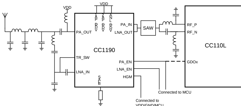
Figure 24: Simplified CC110L-CC1190 Application Circuit
