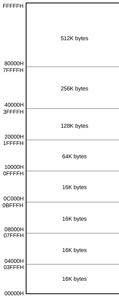
Fig. 10-2 Memory Space
