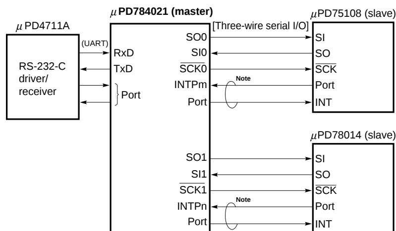
(b) UART + Three-wire serial I/O
