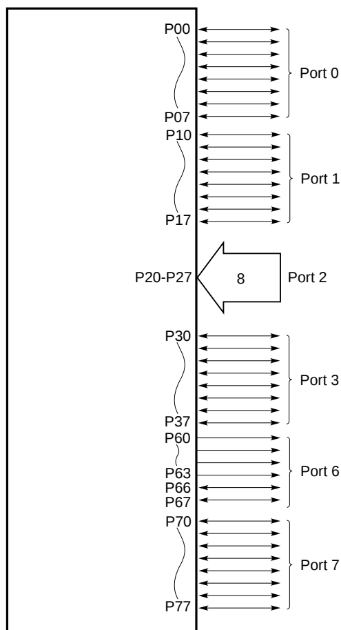
Fig. 8-1 Port Configuration
