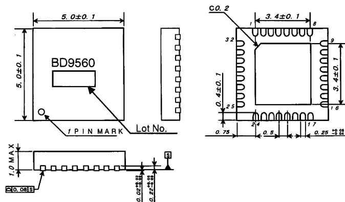
VQFN032V5050
