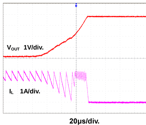
Figure 16. Short Circuit Recovery Waveform
