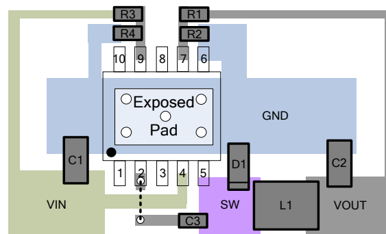
Figure 19. Recommended Layout Diagram (MSOP-10 exposed pad package)
