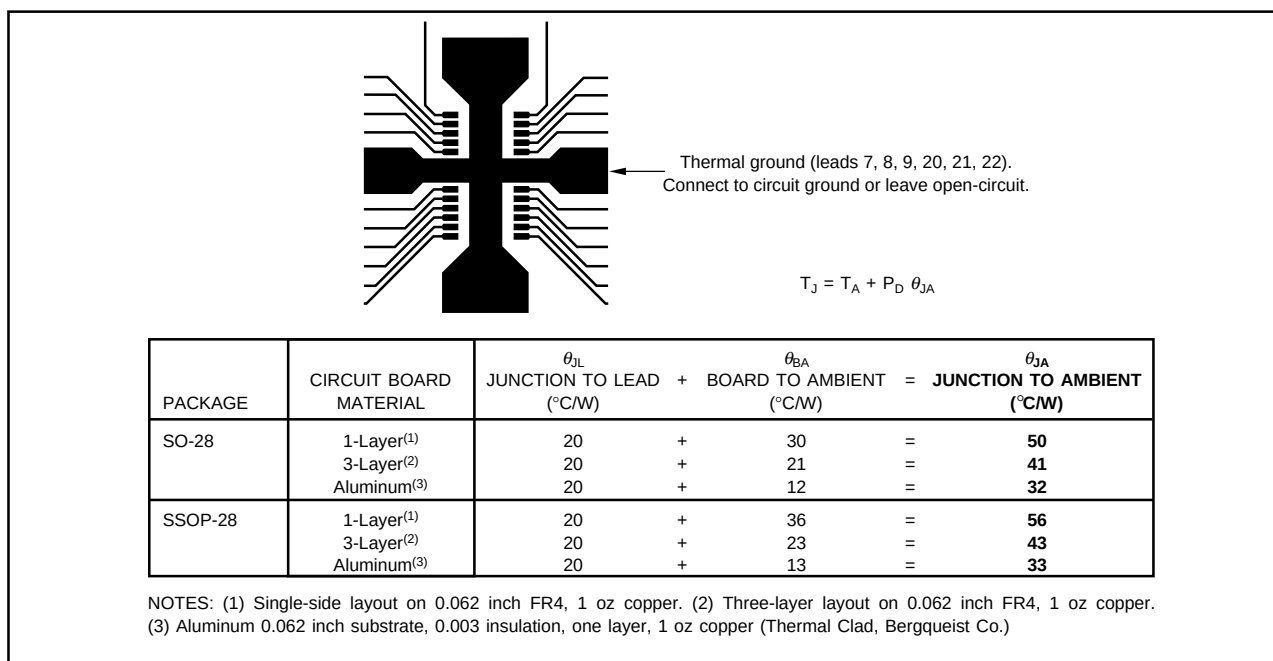
FIGURE 2. Circuit Board Layout.
