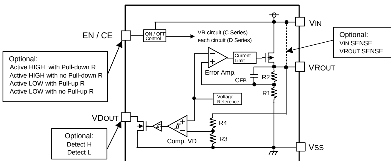
XC6403C, D Series
