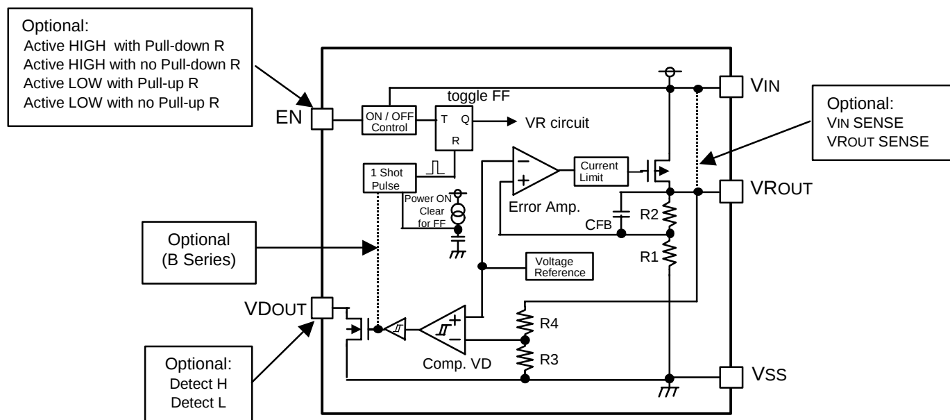
XC6403A, B Series
