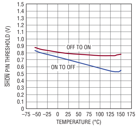
\overline{\text{SHDN}} Pin Threshold
