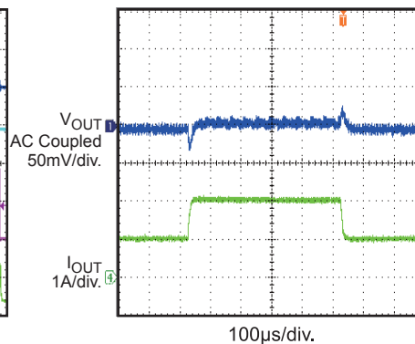
Load Transient I_{OUT} = 1A to 2A , 2.5A/\mu s
