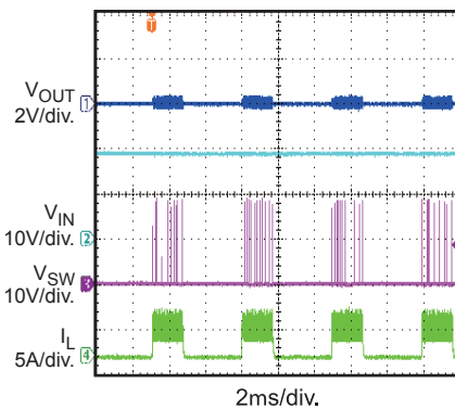
Short Circuit Steady I_{OUT} = 0A
