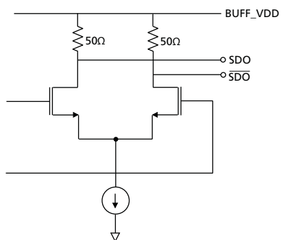
Figure 3-8: SDO/SDO-
