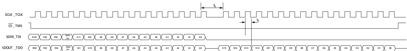
Figure 4-31: Read Mode
