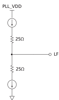
Figure 3-7: Loop Filter
