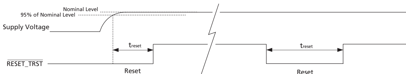
Figure 4-35: Reset Pulse
