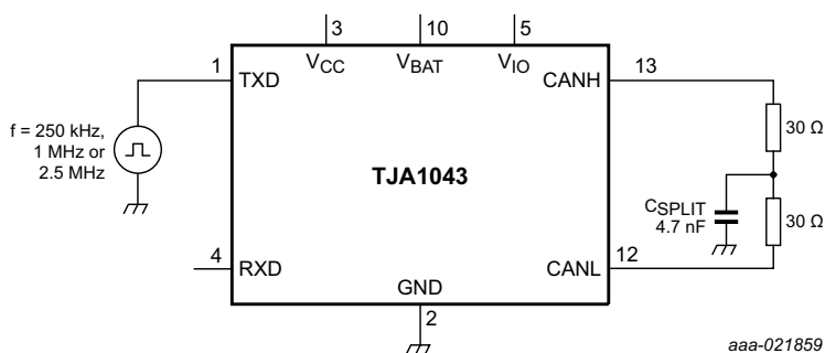
Fig 12. Test circuit for measuring transceiver driver symmetry
