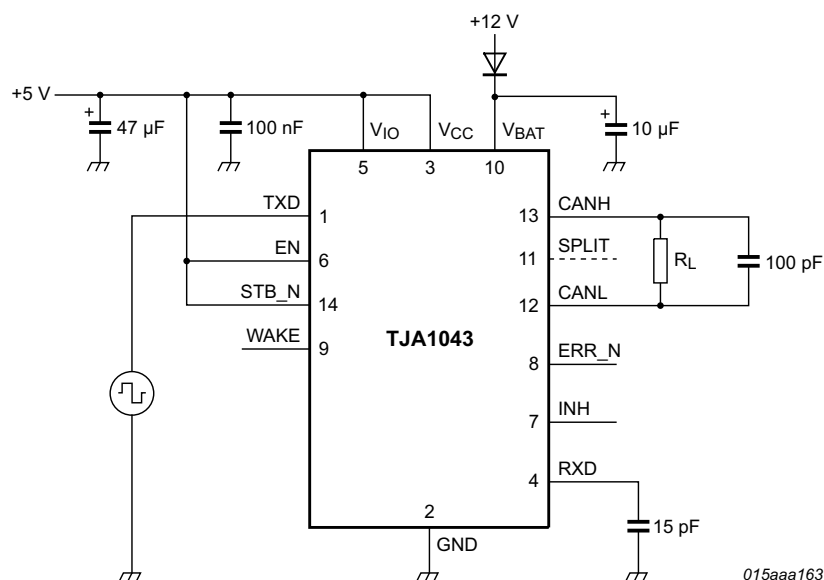
Fig 11. Test circuit for timing characteristics
