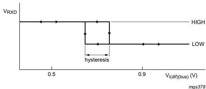
Fig 10. Hysteresis of the receiver
