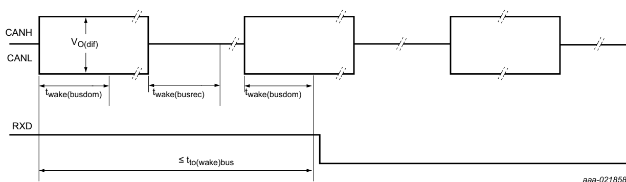
Fig 5. Wake-up timing
