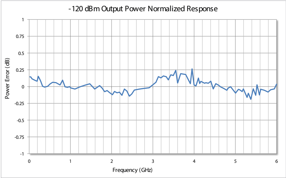
Figure 7. Output power normalized response at –120 dBm.
