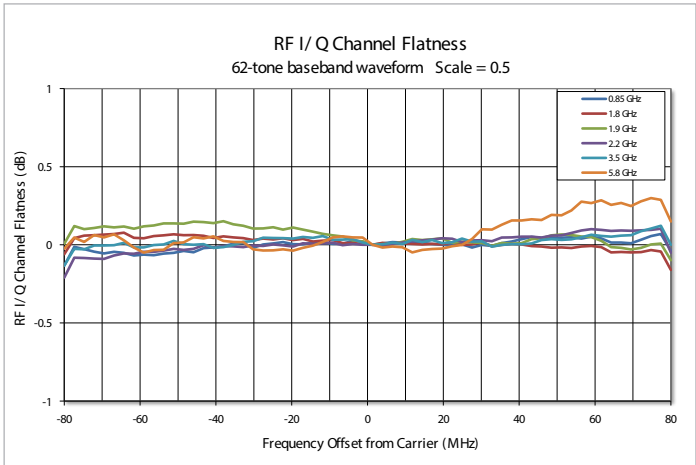
Figure 16. RF I/Q channel flatness at various carrier frequencies.
