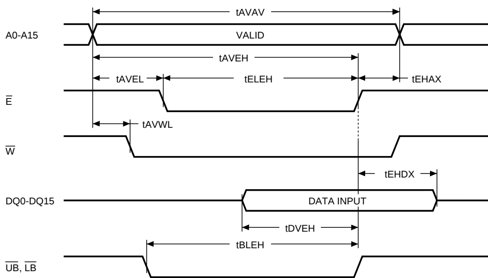
Figure 11. Chip Enable Controlled, Write AC Waveforms
