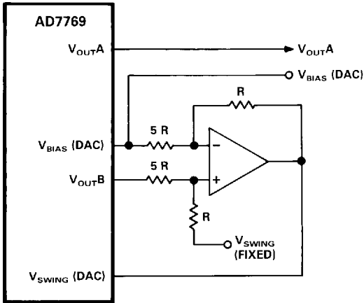
Figure 28. Generating a Software Programmable V_{\text{SWING}} (DAC)
