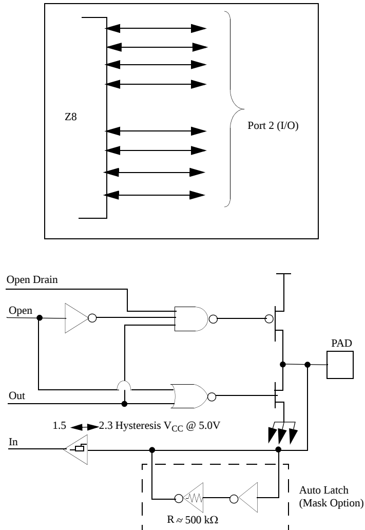
Figure 4. Port 2 Configuration
