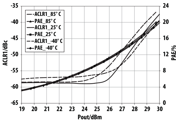
Figure 9. Over-temperature ACLR1, PAE vs Pout @ 2.14 GHz V_{dd} = V_{ddBias} = 5.0\text{ V} operating voltage
