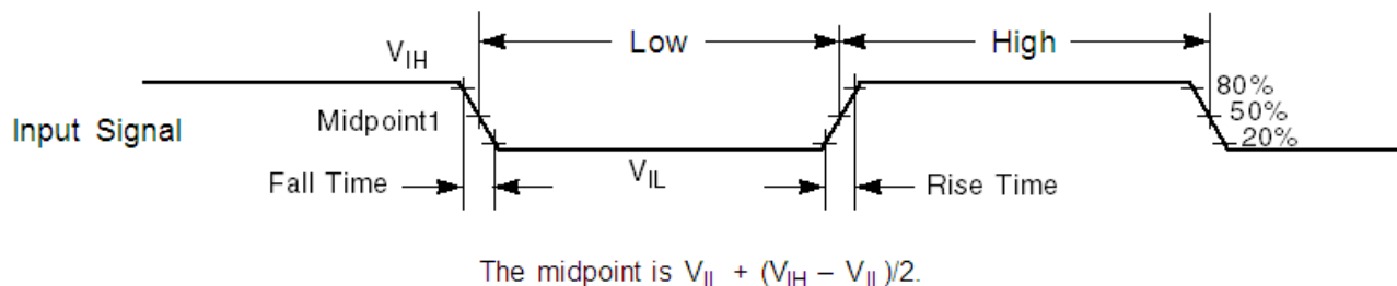
Figure 6. Input signal measurement reference
