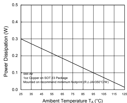
Maximum Power Dissipation of SOT 23
