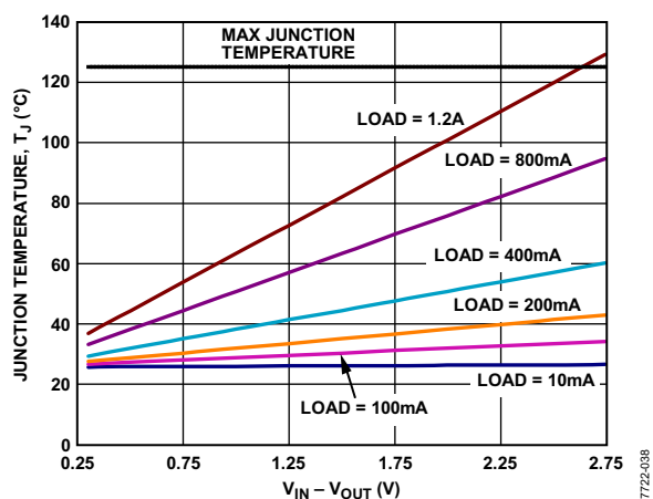
图42. 500 mm² PCB覆铜, T_B = 25^\circ\text{C} , LFCSP
