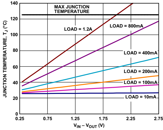
图36. 6400 mm² PCB覆铜, T_A = 25^\circ\text{C} , LFCSP
