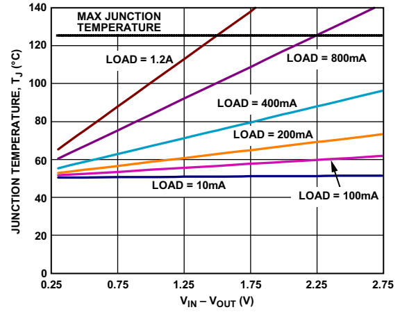
图39. 6400 mm² PCB覆铜, T_A = 50^\circ\text{C} , LFCSP
