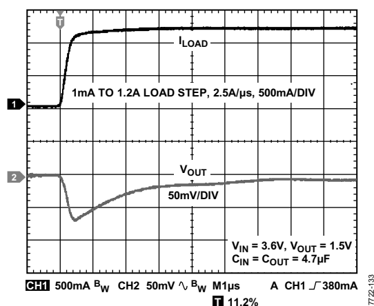
图33. 输出瞬态响应( C_{\text{OUT}} = 4.7\ \mu\text{F} )
