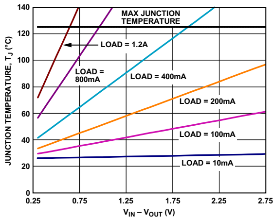
图38. 0 mm² PCB覆铜, T_A = 25^\circ\text{C} , LFCSP
