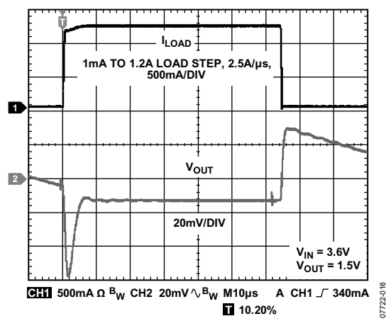
图16. 负载瞬态响应( C_{\text{IN}} = 22 \mu\text{F} , C_{\text{OUT}} = 22 \mu\text{F} )
