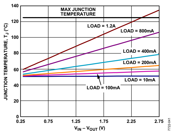
图45. 1000 mm² PCB覆铜, T_B = 50^\circ\text{C} , LFCSP
