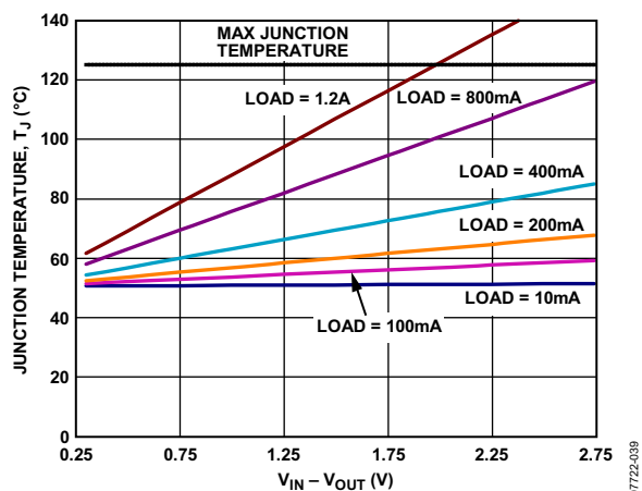
图43. 500 mm² PCB覆铜, T_B = 50^\circ\text{C} , LFCSP
