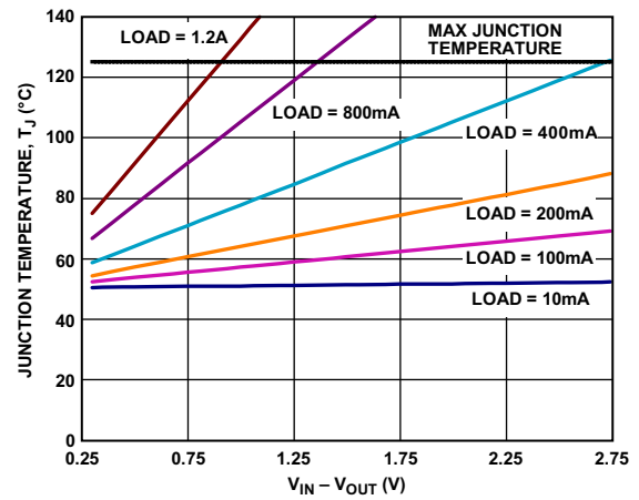
图40. 500 mm² PCB覆铜, T_A = 50^\circ\text{C} , LFCSP
