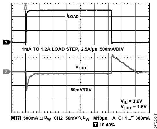
图15. 负载瞬态响应( C_{\text{IN}} = 4.7 \mu\text{F} , C_{\text{OUT}} = 4.7 \mu\text{F} )
