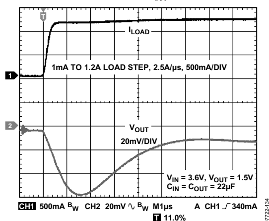
图34. 输出瞬态响应( C_{\text{OUT}} = 22\ \mu\text{F} )
