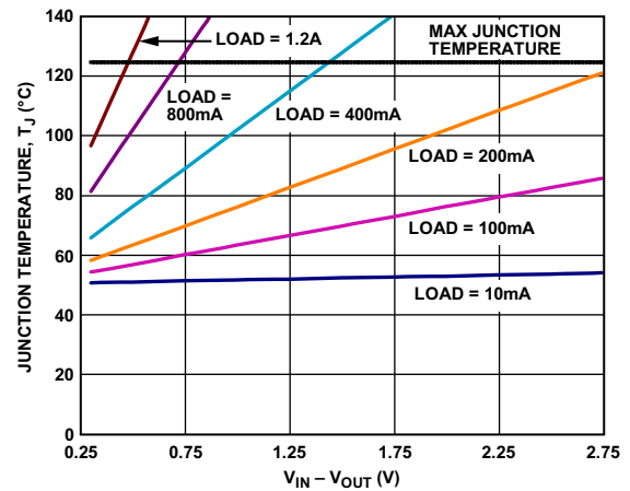
图41. 0 mm² PCB覆铜, T_A = 50^\circ\text{C} , LFCSP
