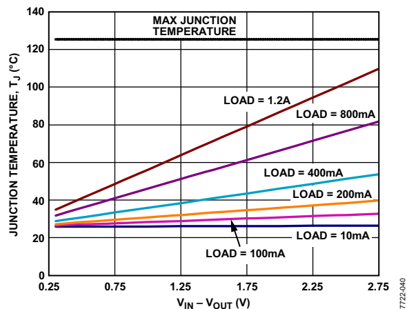
图44. 1000 mm² PCB覆铜, T_B = 25^\circ\text{C} , LFCSP
