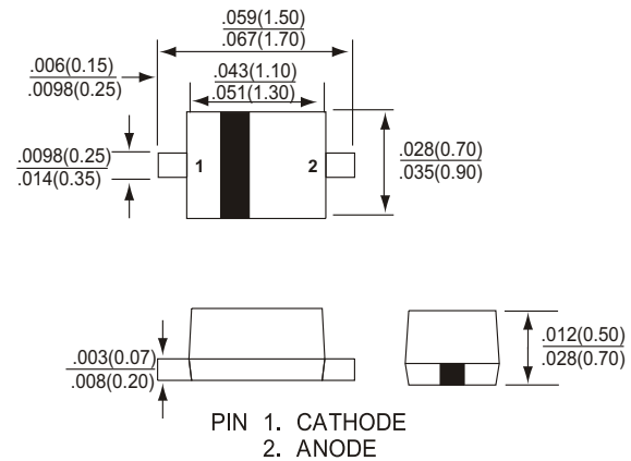
SOD-523
