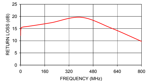
ADT1-1WT INPUT RETURN LOSS
