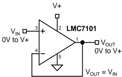
Figure 4. Voltage Follower
