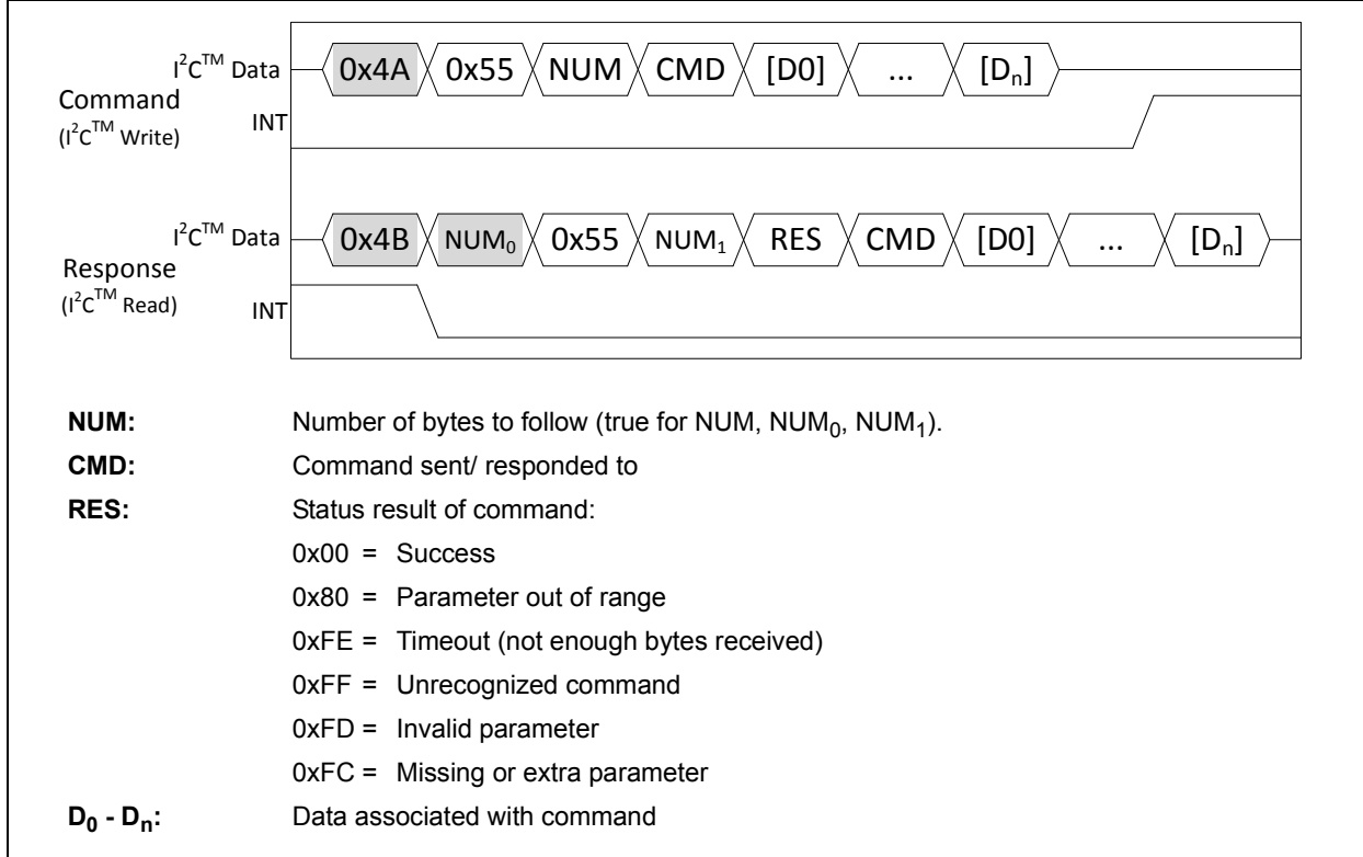
FIGURE 6-5: COMMAND PROTOCOL
