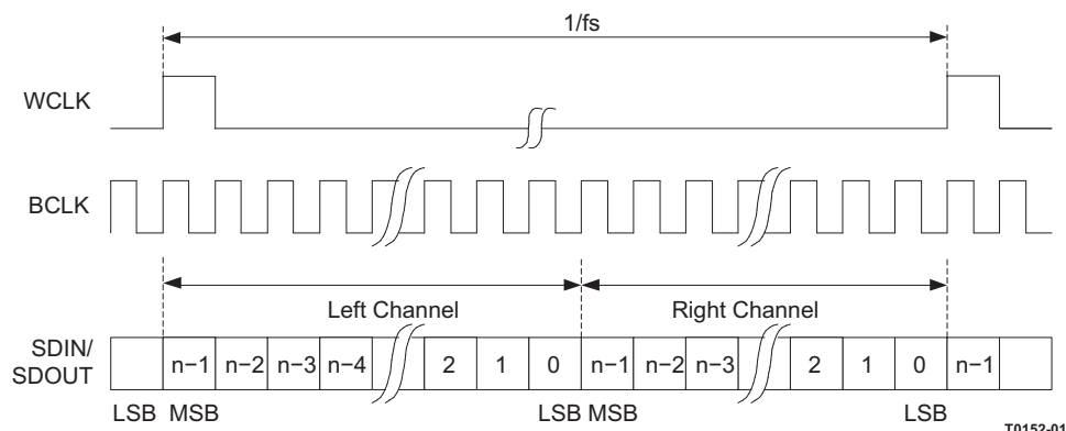
Figure 23. DSP Serial Bus Mode Operation
