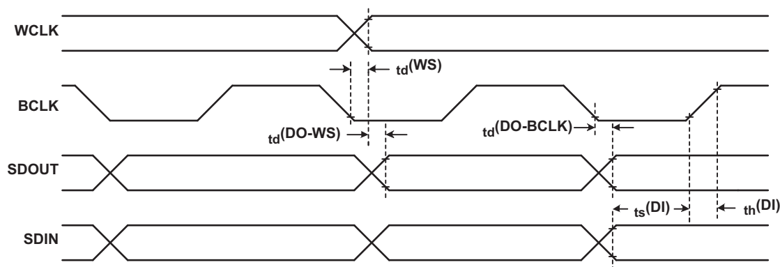
Figure 1. I 2 S/LJF/RJF Timing in Master Mode
