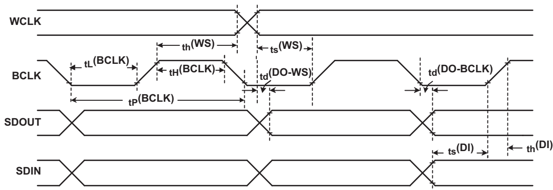
Figure 3. I²S/LJF/RJF Timing in Slave Mode
