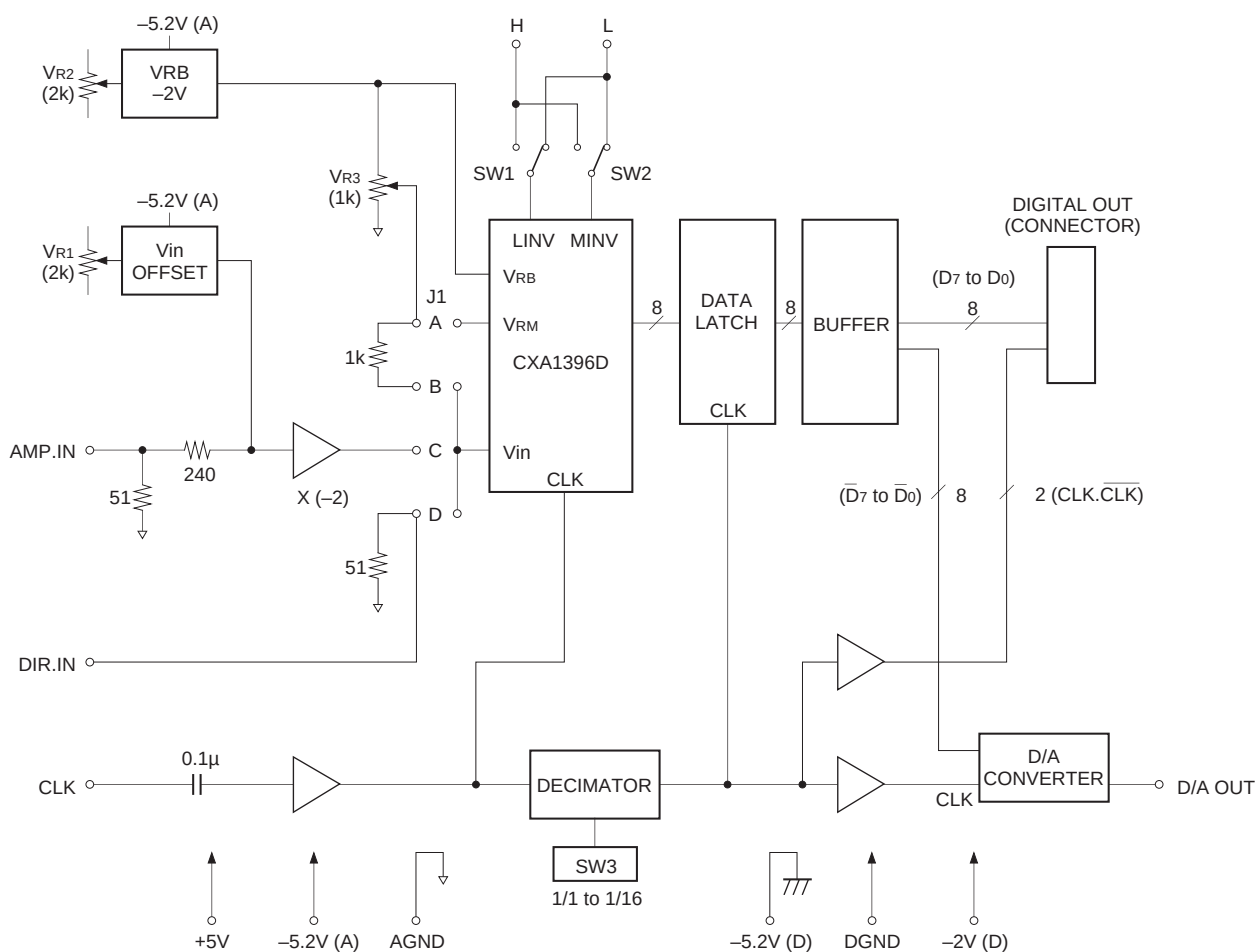
Fig. 1. Block Diagram
