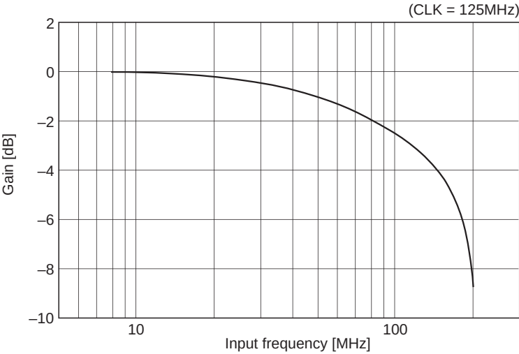
Fig. 5. Gain vs. Input frequency
