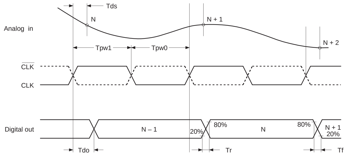
Timing diagram
