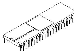
42 pin DIP (Ceramic)
