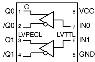
8-Pin MLF®
