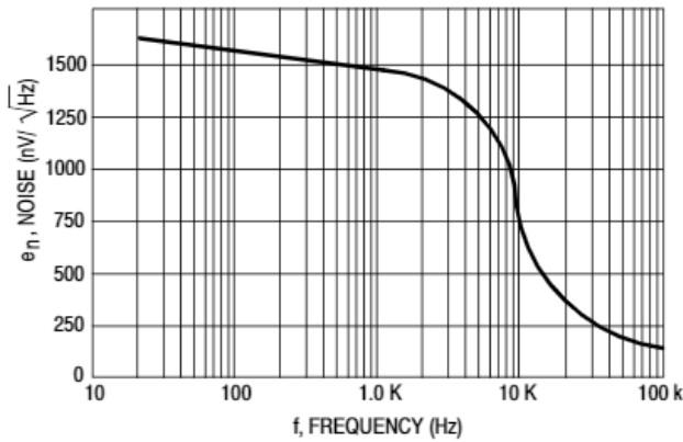
Figure 12. Noise Voltage
