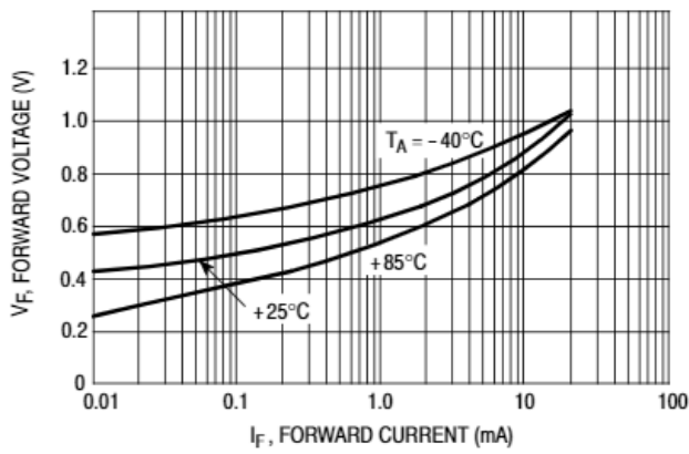
Figure 10. Forward Characteristics
