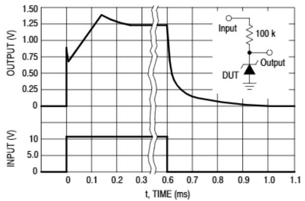
Figure 7. Response Time
