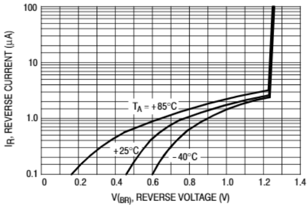
Figure 2. Reverse Characteristics
