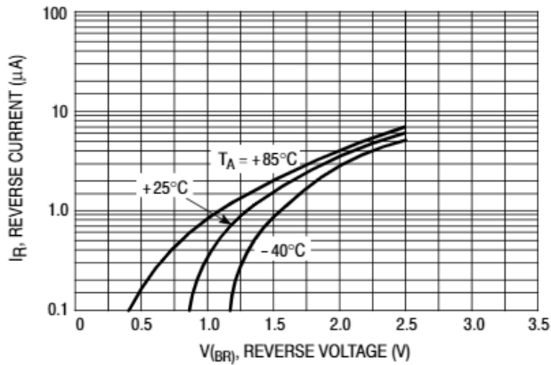
Figure 8. Reverse Characteristics
