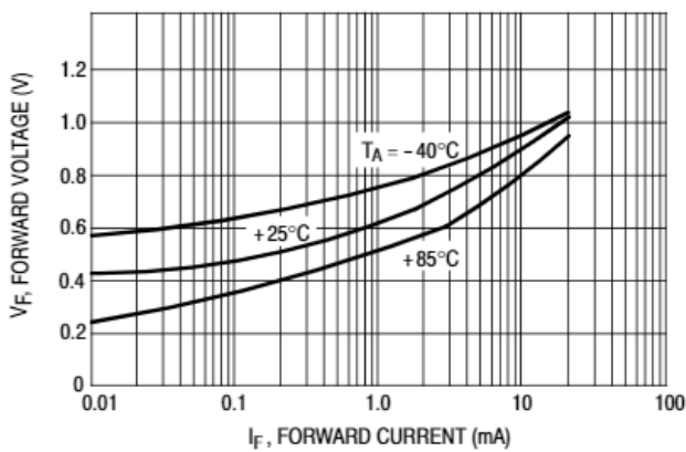
Figure 4. Forward Characteristics
