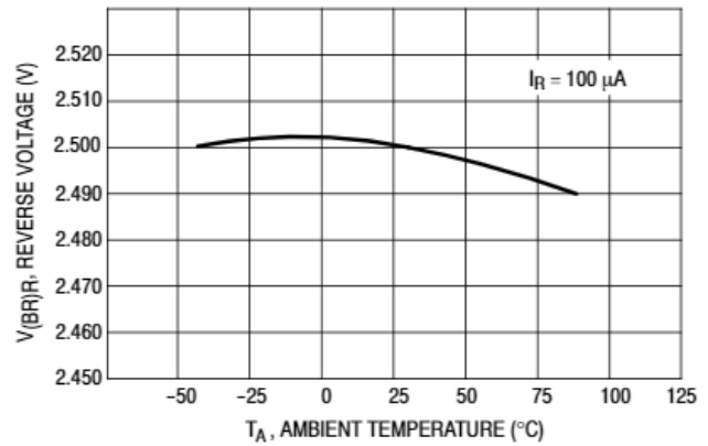
Figure 11. Temperature Drift
