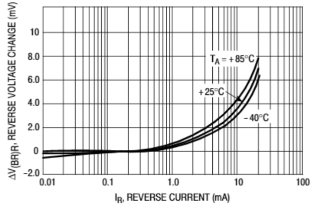
Figure 3. Reverse Characteristics
