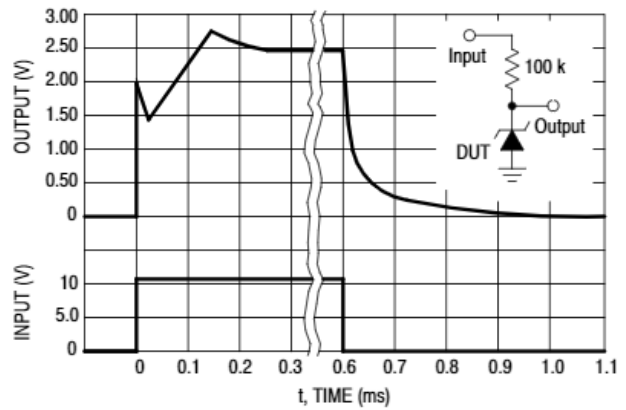
Figure 13. Response Time
