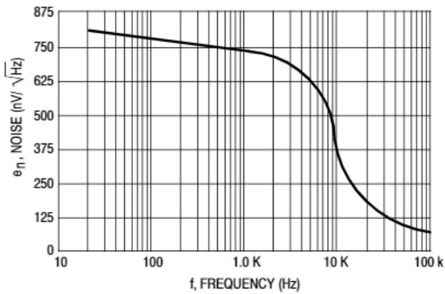
Figure 6. Noise Voltage
