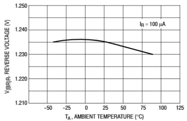
Figure 5. Temperature Drift
