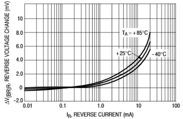
Figure 9. Reverse Characteristics
