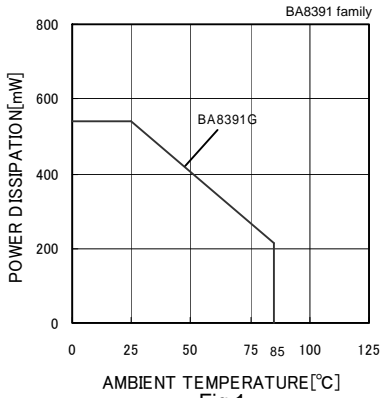
Fig.1 Derating Curve
