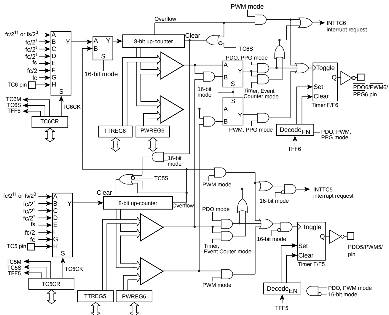
Figure 11-1 8-Bit TimerCounter 5, 6
