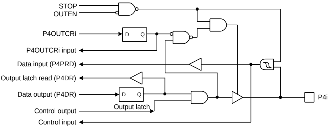
Figure 5-6 Port 4
