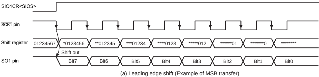
(a) Leading edge shift (Example of MSB transfer)
