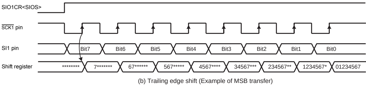
(b) Trailing edge shift (Example of MSB transfer)
