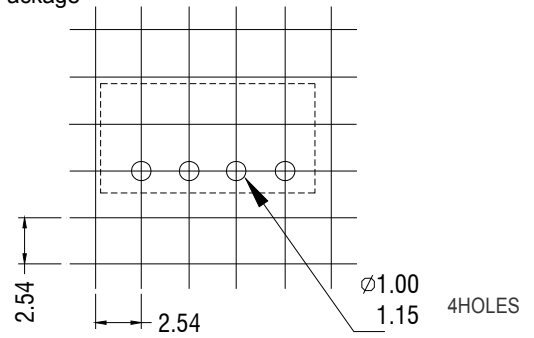
4 Pin SIP Package
