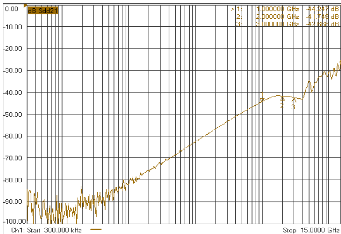
Crosstalk
