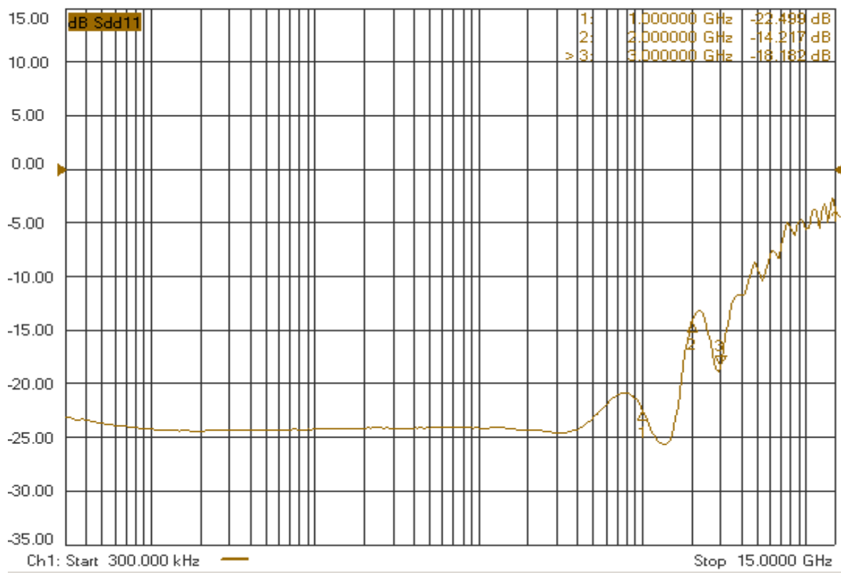
Return Loss
