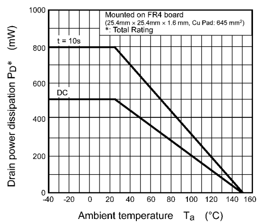
Fig. 7.12 P_D - T_a
