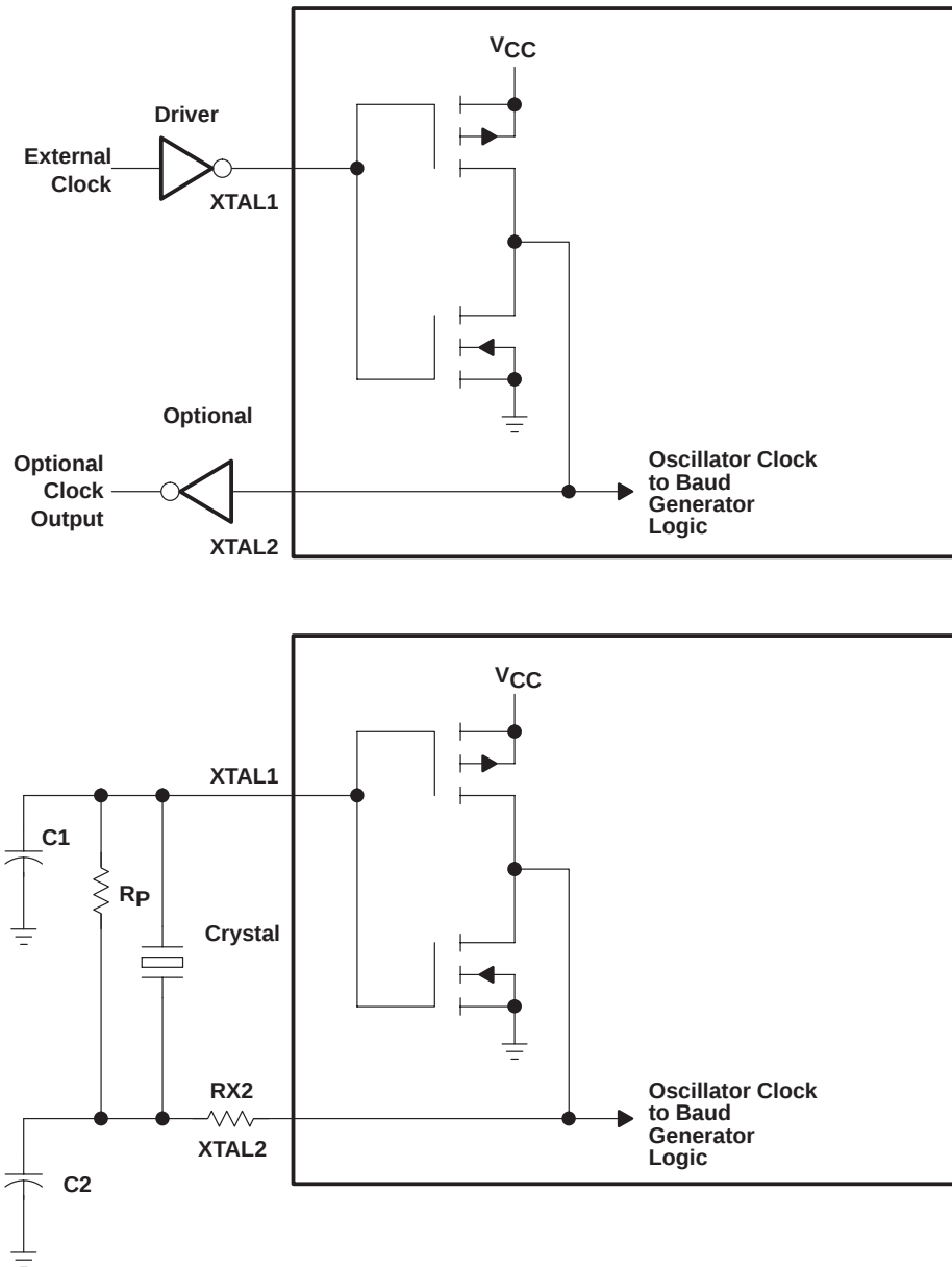
TYPICAL CRYSTAL OSCILLATOR NETWORK
