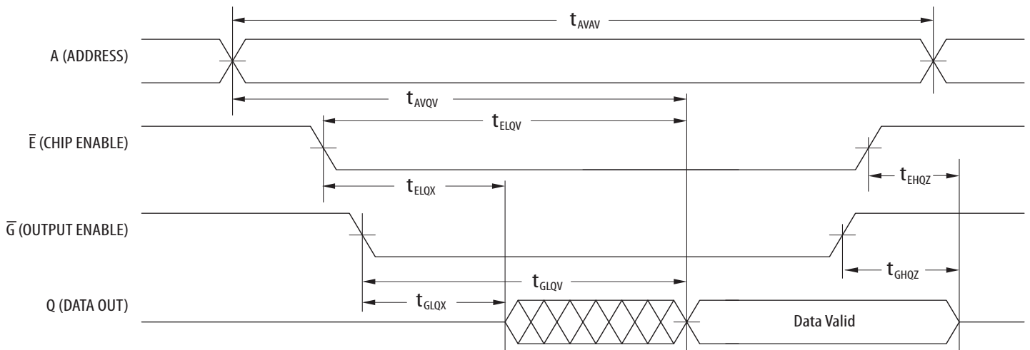
Figure 3.3B Read Cycle 2
