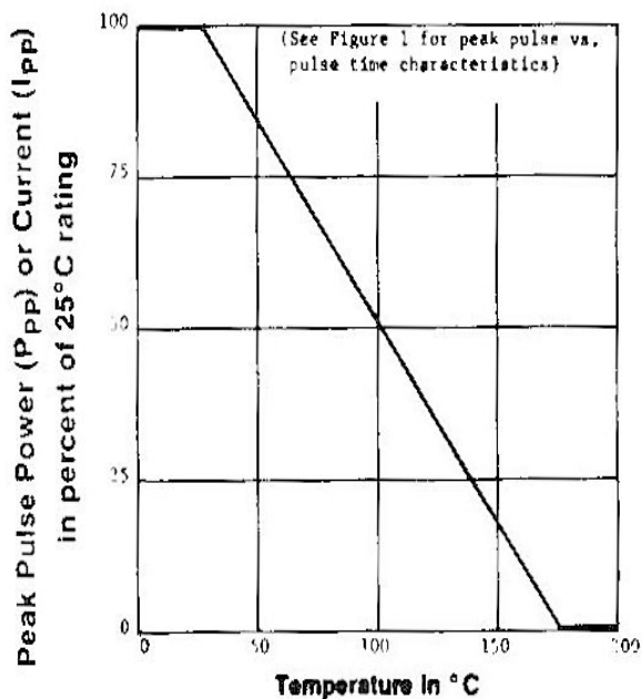
Figure 3 Derating Curve
